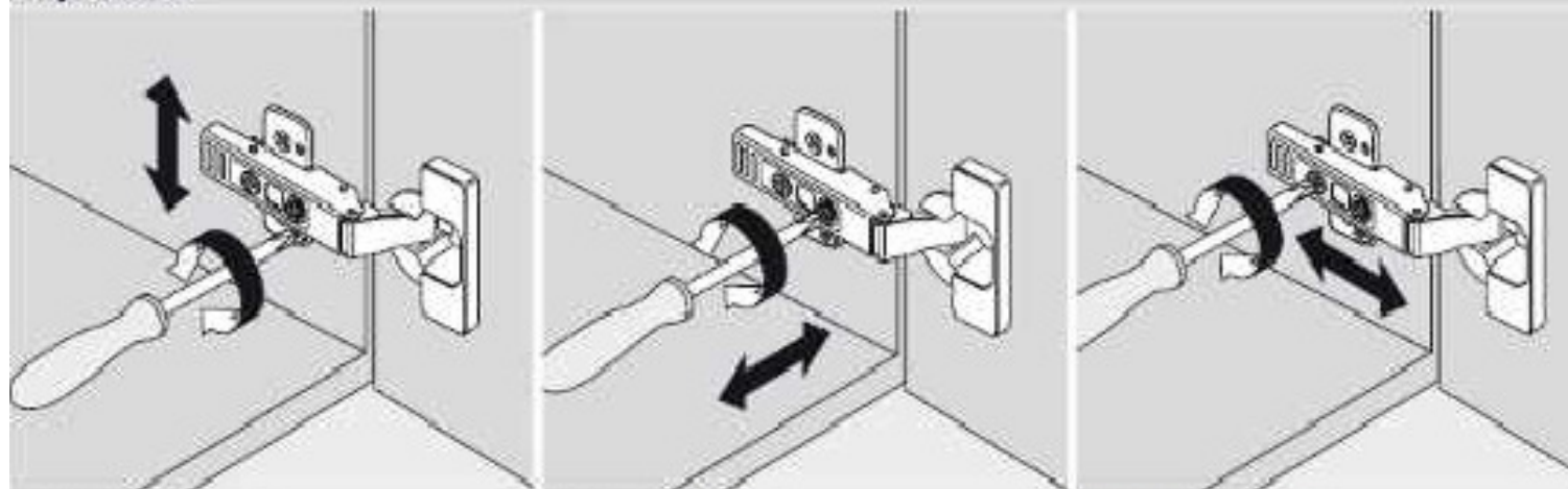
Height adjustment
